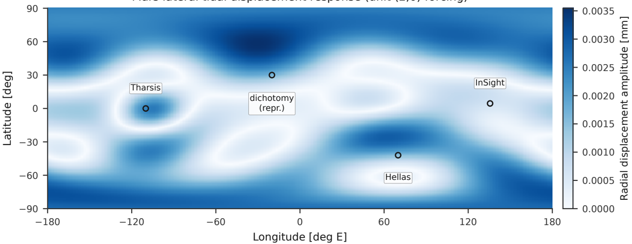
Mars lateral tidal displacement response (unit (2,0) forcing)
