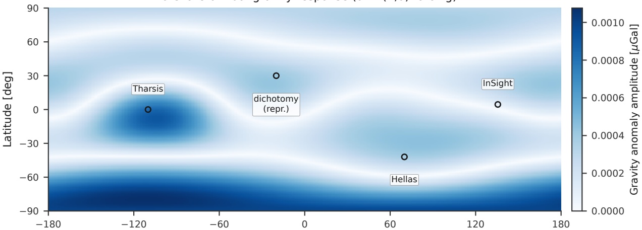
Mars lateral tidal gravity response (unit (2,0) forcing)
