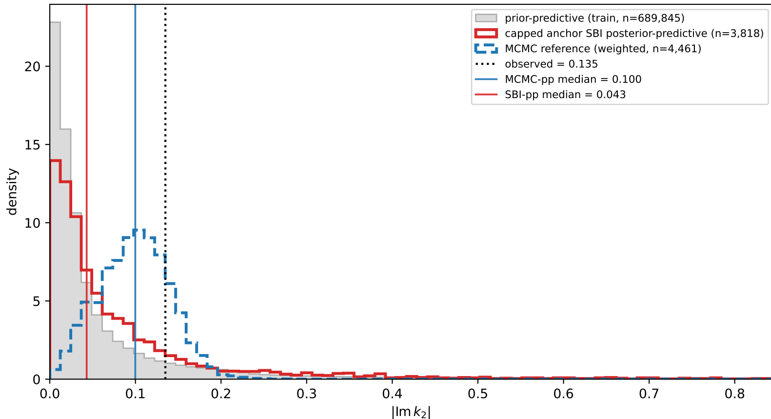
Titan NH3 joint — capped anchor |Im\,k_2| pushforward shape (concentration-failure vs wrong-mode diagnostic)
