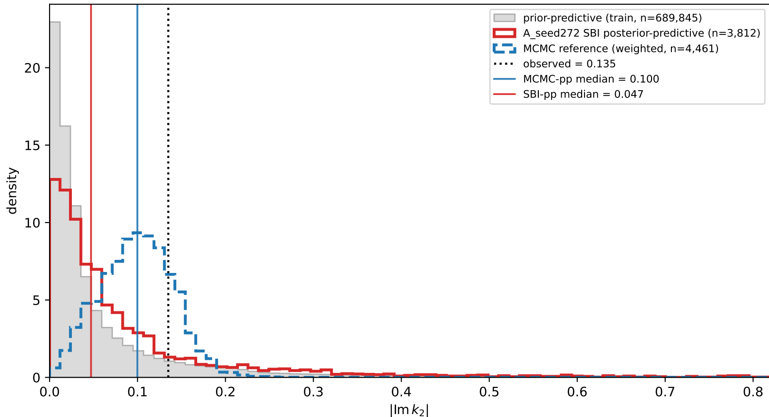
Titan NH3 joint — A_seed272 |Im\,k_2| pushforward shape (concentration-failure vs wrong-mode diagnostic)
