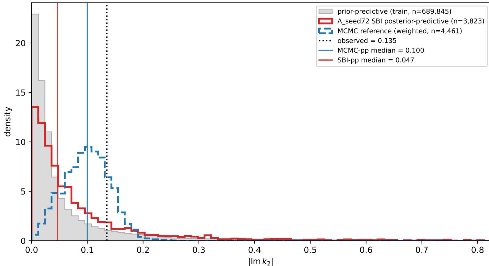
Titan NH3 joint — A_seed72 |Im k_2| pushforward shape (concentration-failure vs wrong-mode diagnostic)
