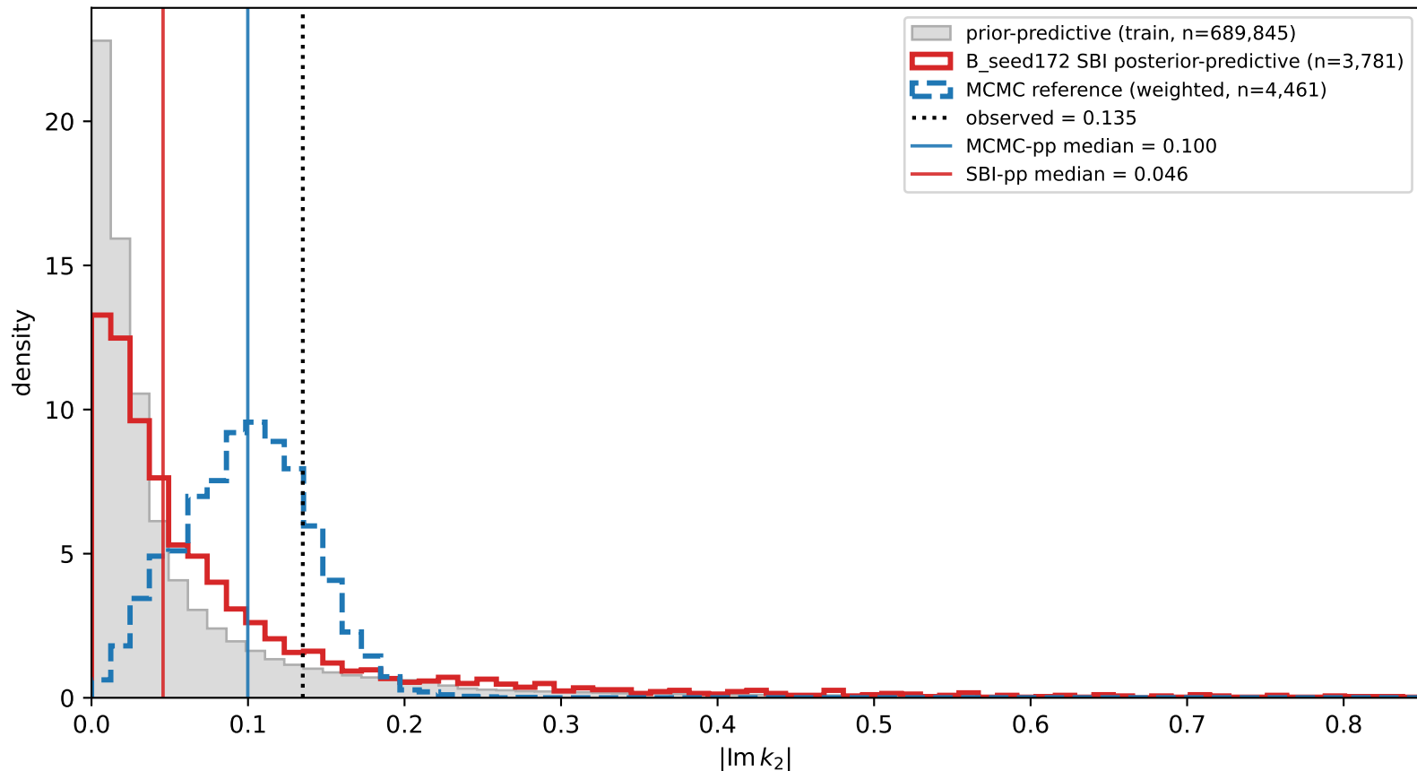
Titan NH3 joint — B_seed172 |\text{Im } k_2| pushforward shape (concentration-failure vs wrong-mode diagnostic)
