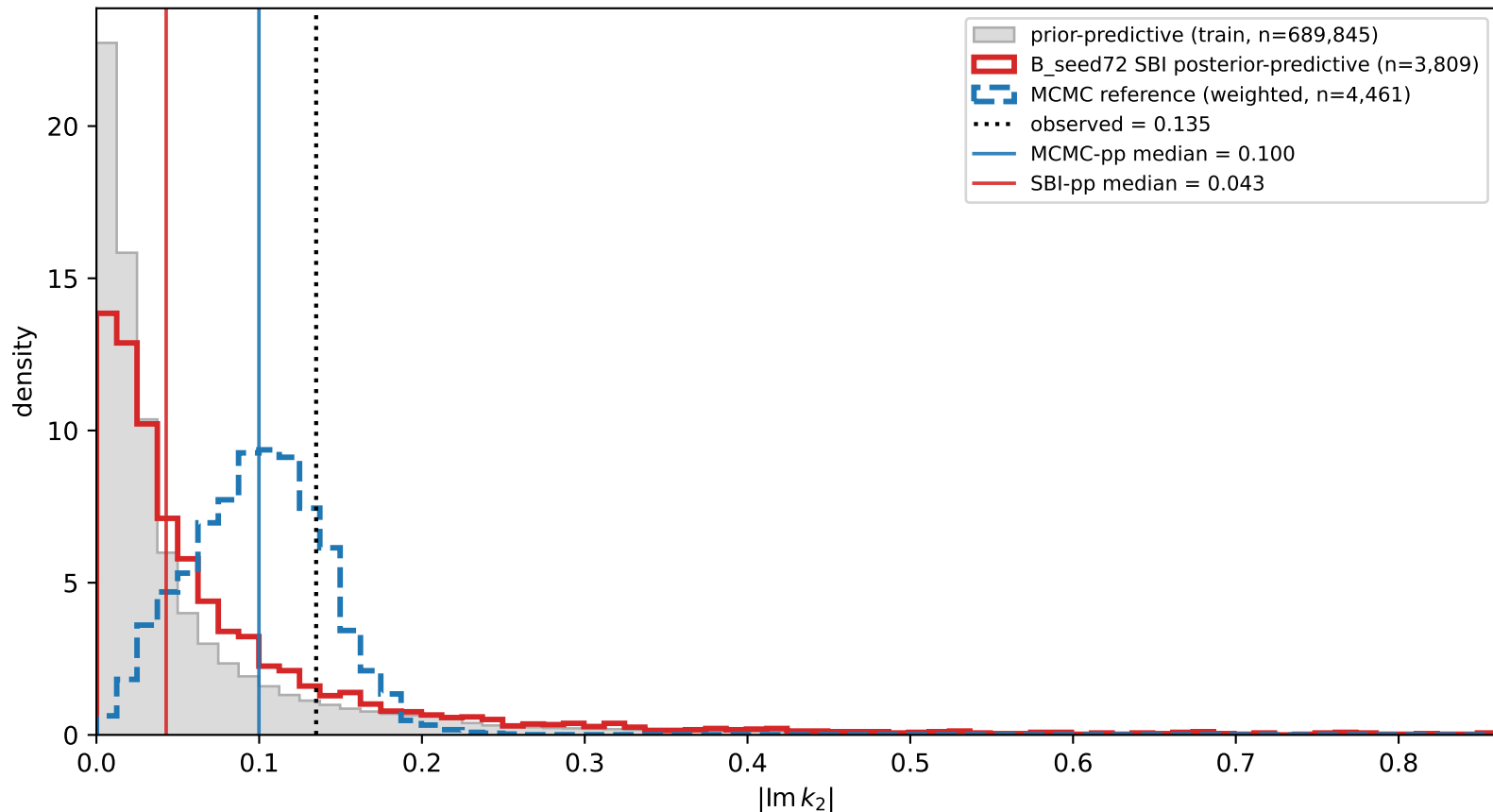
Titan NH3 joint — B_seed72 |Im k_2| pushforward shape (concentration-failure vs wrong-mode diagnostic)
