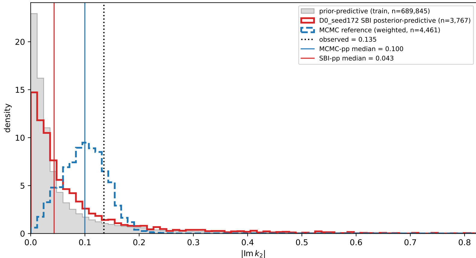
Titan NH3 joint — D0_seed172 |Im k_2| pushforward shape (concentration-failure vs wrong-mode diagnostic)
