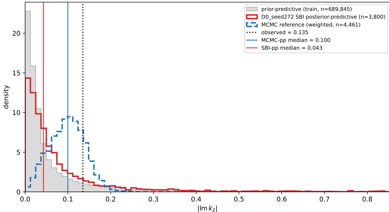
Titan NH3 joint — D0_seed272 |Im k_2| pushforward shape (concentration-failure vs wrong-mode diagnostic)
