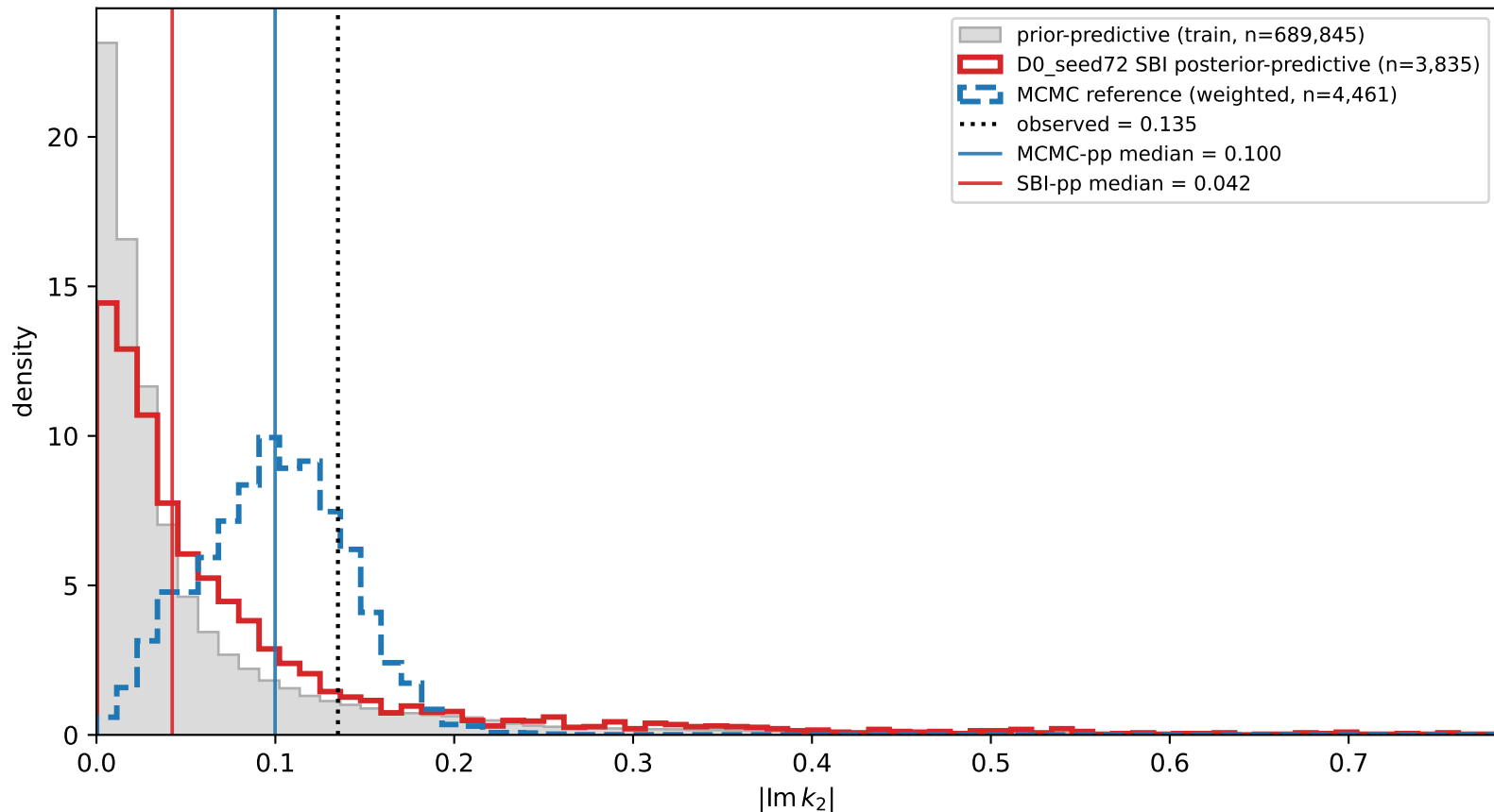
Titan NH3 joint — D0_seed72 |\text{Im } k_2| pushforward shape (concentration-failure vs wrong-mode diagnostic)
