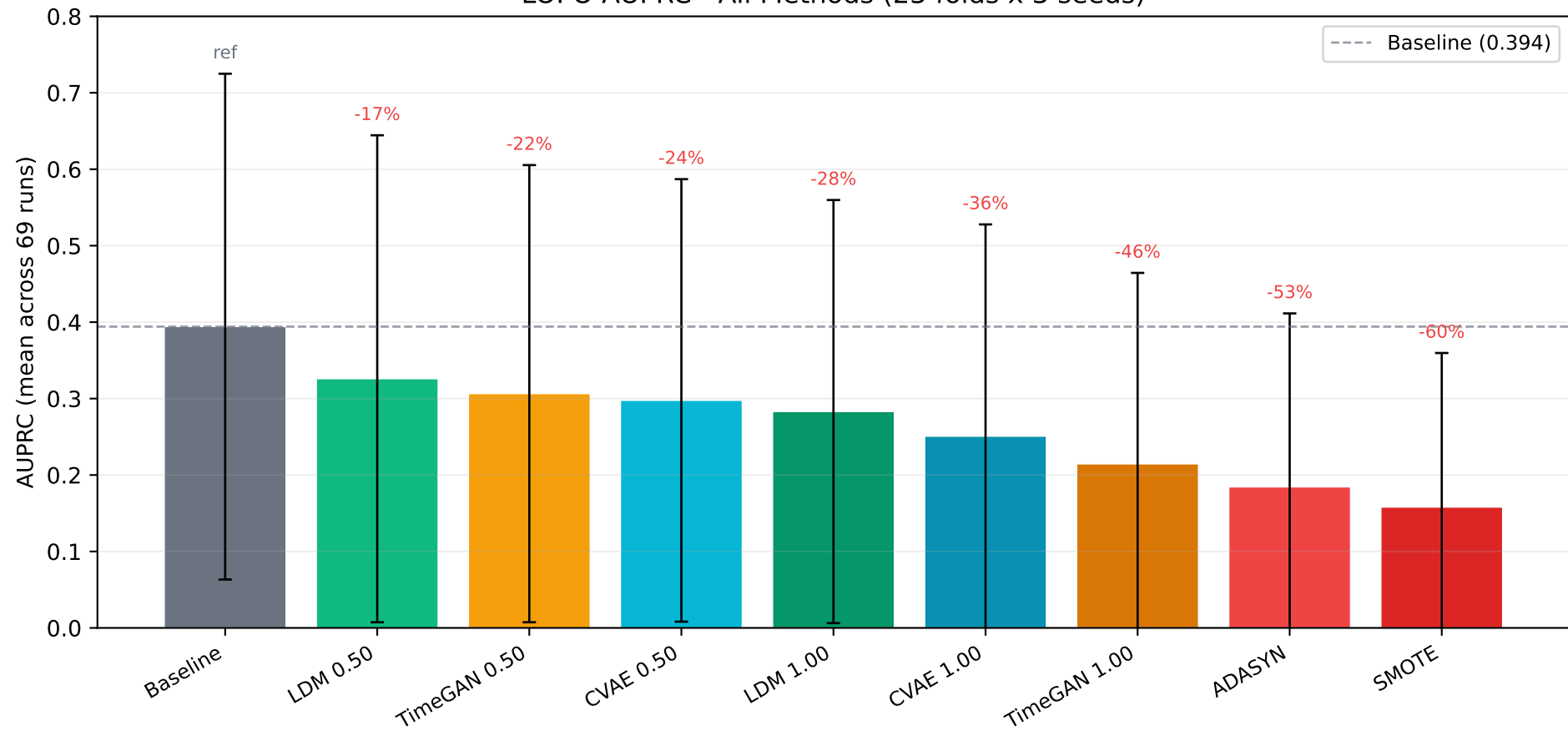
LOPO AUPRC - All Methods (23 folds x 3 seeds)
