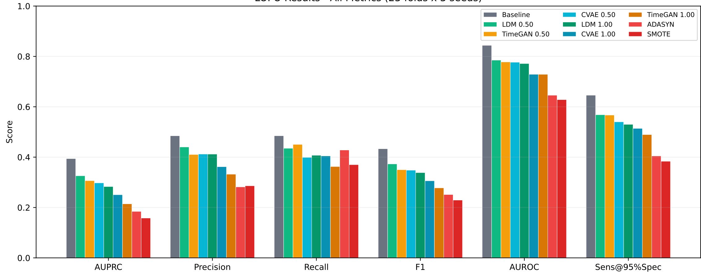
LOPO Results - All Metrics (23 folds x 3 seeds)
