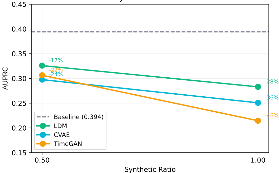
Ratio Sensitivity - All Generators Under LOPO
