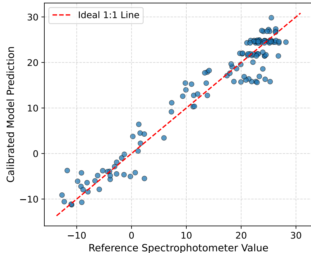
a* (Green-Red) ( R^2 = 0.942 , RMSE = 3.00)
