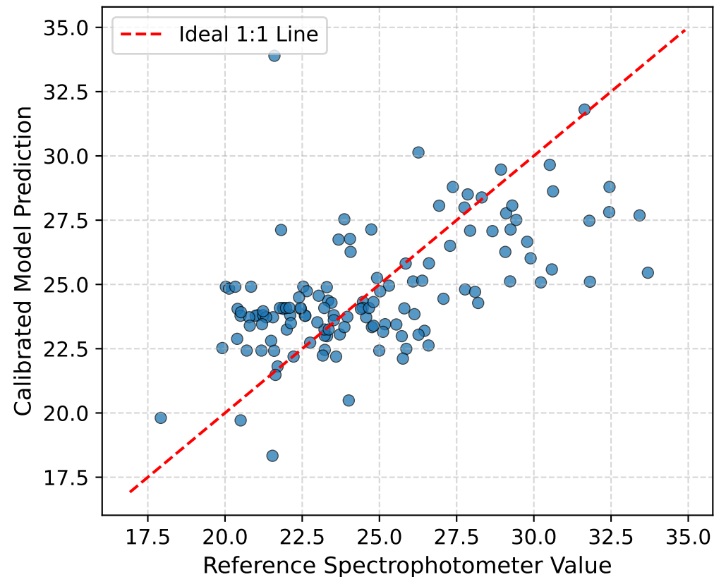
b* (Blue-Yellow) ( R^2 = 0.328 , RMSE = 2.77)
