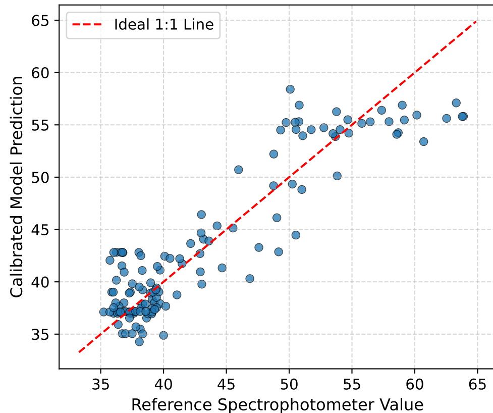
L* (Lightness) ( R^2 = 0.827 , RMSE = 3.27)
