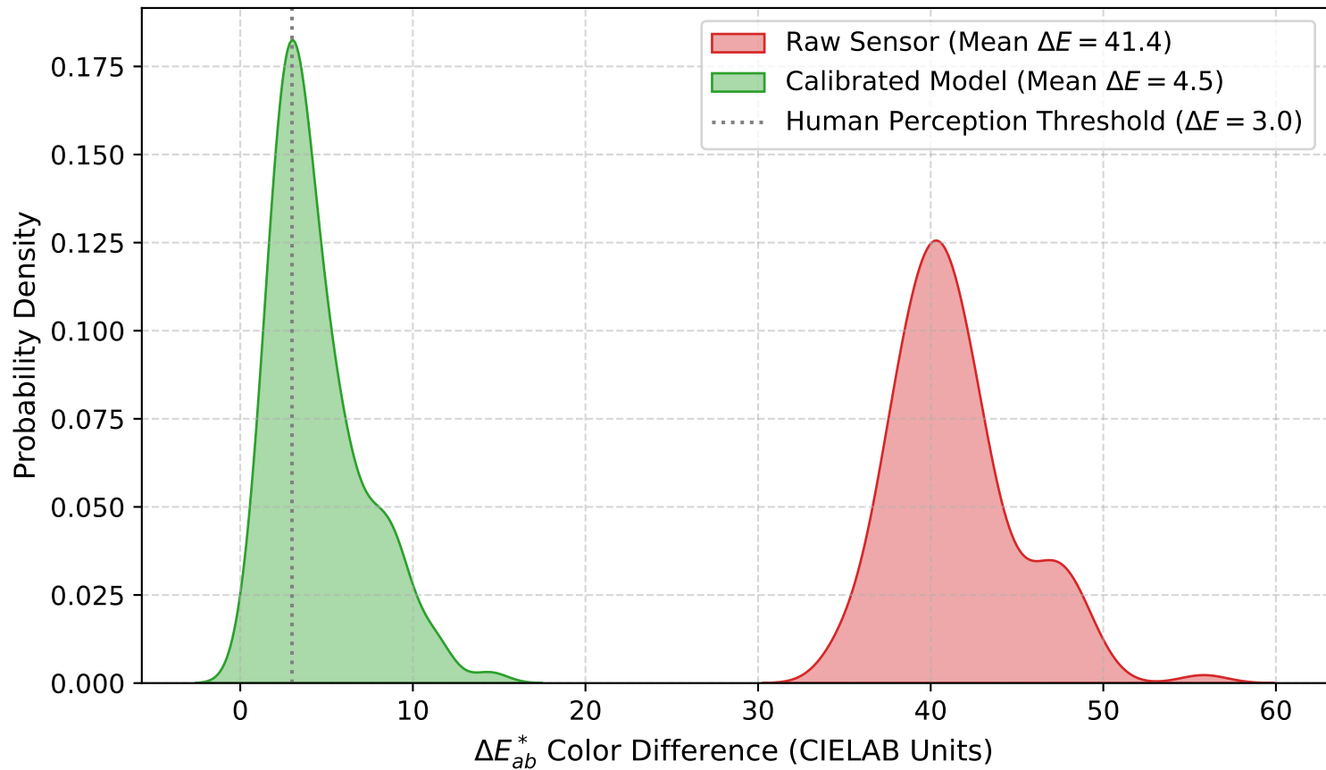
Colorimetric Error Distribution Before and After Calibration
