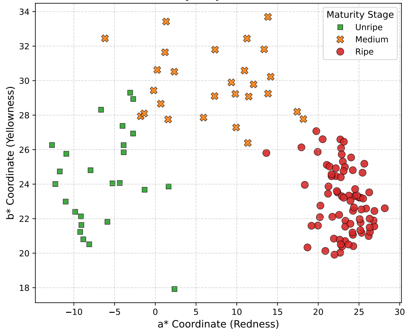
Chromaticity Projection ( a^* vs. b^* )
