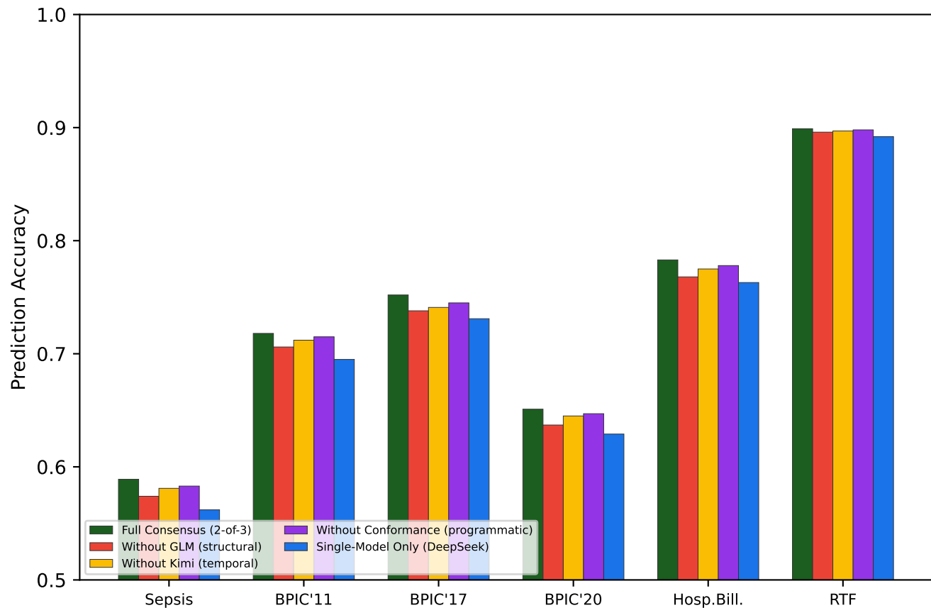
Ablation Study: Contribution of Each Verification Component Across Six Event Logs (2.0x)
