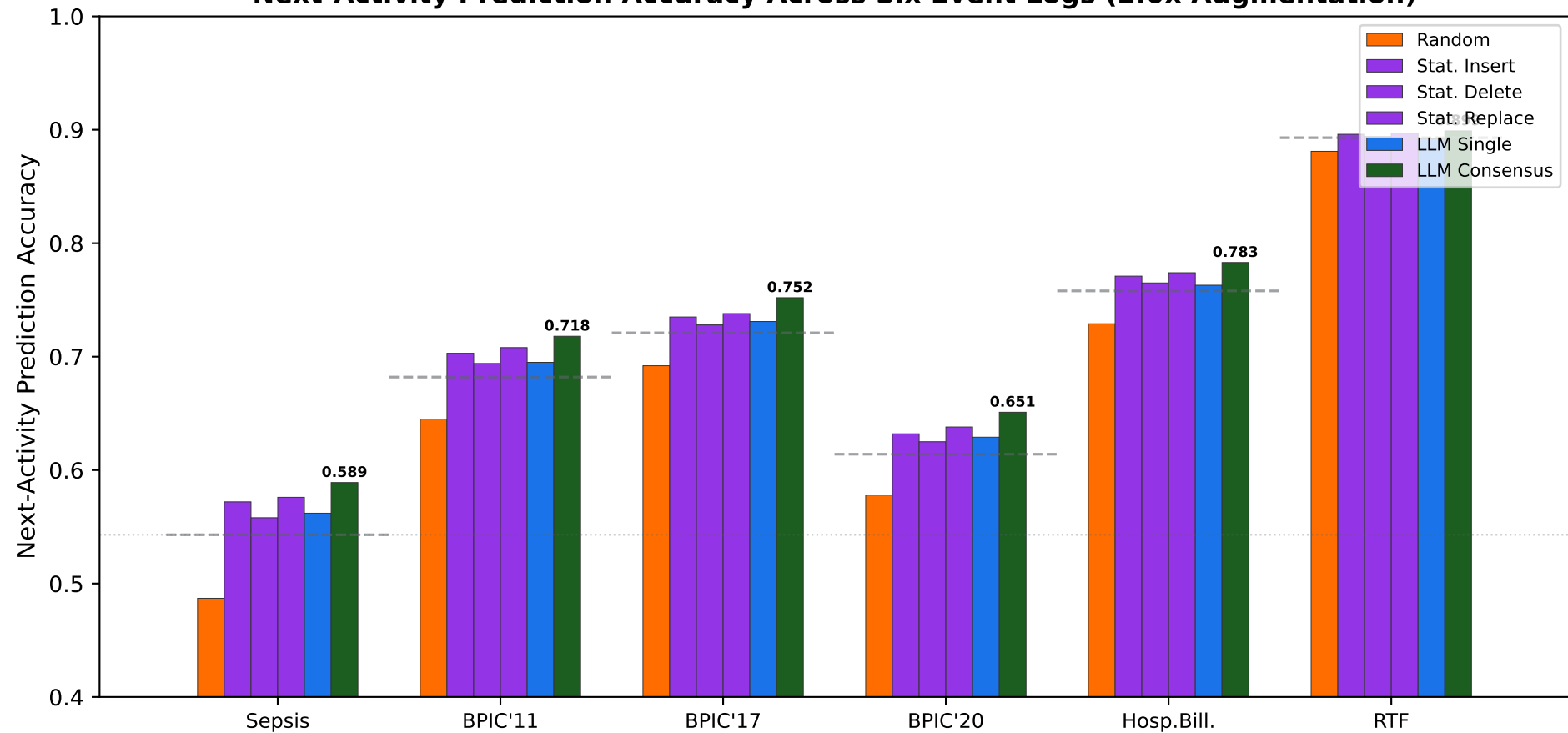
Next-Activity Prediction Accuracy Across Six Event Logs (2.0x Augmentation)
