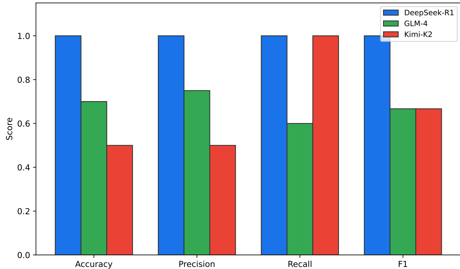
Verifier Role: Trace Classification Performance
