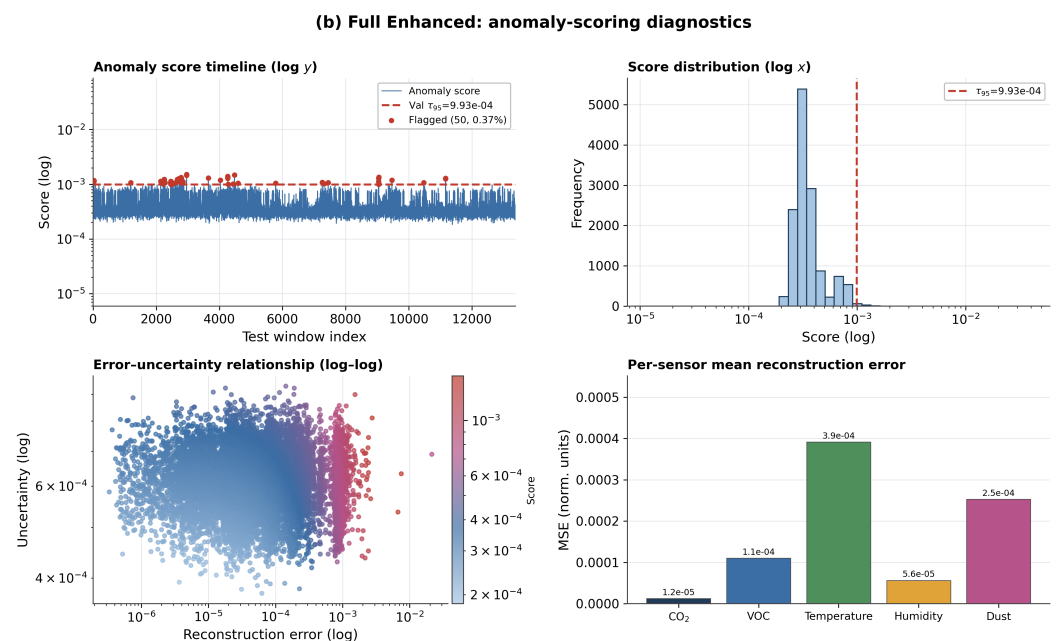
(b) Full Enhanced (Proposed Model): \tau_{95} = 9.93 \times 10^{-4} , 50 flagged (0.37%).
