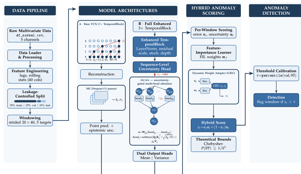
Figure 1. End-to-end architecture of the proposed uncertainty-aware TCN framework, organised as a four-stage pipeline: Data Pipeline (loading, leakage-controlled split, windowing) → Model Architectures (Base TCN and Full Enhanced) → Hybrid Anomaly Scoring → Anomaly Detection . The key backbone components are broken down inline: the Base TCN’s dilated causal convolution stack (kernel k=2 , dilations d_l=\{1, 2, 4\} , receptive field RF=8 ); the red path traces the dilated dependencies feeding the output \hat{y}_t , MC-dropout inference ( M stochastic passes \Rightarrow predictive mean \hat{y}_t and per-sensor epistemic \sigma_t ), the AUA (4-head attention element-wise modulated by the uncertainty gate g_t=1/(1+\sigma_t) ), and the Dynamic Weight Adapter (GRU over e_t, u_t producing the learned weight \alpha_t ). Dark boxes mark the framework’s contributed components; the dashed red arrow marks the uncertainty-to-attention coupling that distinguishes this work from approaches that apply uncertainty only post hoc; detection via validation-calibrated thresholding terminates the pipeline.
