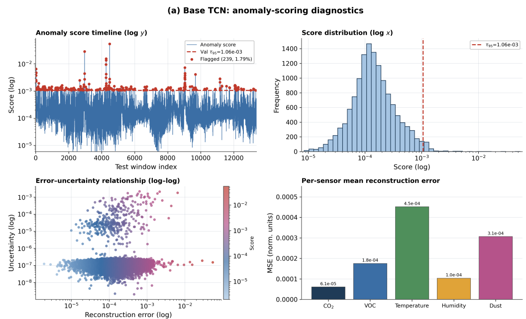
(a) Base TCN: \tau_{95} = 1.06 \times 10^{-3} , 239 flagged (1.79%).
