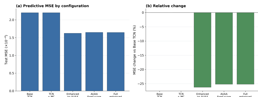
Figure 5. Ablation summary on the held-out test split: the auxiliary objectives (Configuration 3) deliver the largest MSE reduction, which AUAA (Configuration 4) and the full integration (Configuration 5) preserve.
