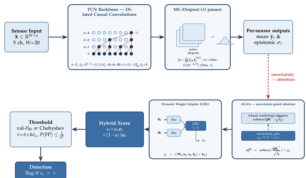
Figure 1. End-to-end architecture of the proposed uncertainty-aware TCN framework, drawn as a single serpentine flow. The top row is the uncertainty backbone with its breakdown illustrations embedded inline: the TCN backbone with its dilated causal convolution stack (kernel k=2 , dilations d_l=2^{l-1}=\{1,2,4\} , receptive field RF=8 ; the red path traces the dilated dependencies feeding the output \hat{y}_t ), MC-dropout inference ( M stochastic forward passes \Rightarrow predictive mean \hat{y}_t and per-sensor epistemic standard deviation \sigma_t ), and the per-sensor outputs. The bottom row applies the contributed components (dark boxes): the AUAA uncertainty-gated attention, the Dynamic Weight Adapter ( \alpha_t ), the hybrid score, the distribution-free Chebyshev/percentile threshold, and detection. Solid navy arrows denote the forward flow; the dashed red arrow marks the uncertainty-to-attention coupling that distinguishes this work from approaches that apply uncertainty only post hoc.
