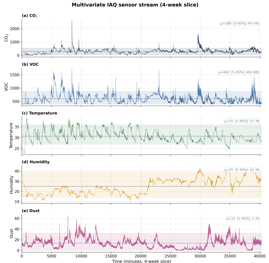
Figure 3. Multivariate indoor air quality sensor stream over a 4-week slice. Panels (a)–(e) show CO 2 , VOC, temperature, humidity, and dust, each overlaid with its mean (dashed) and 5th–95th percentile band (shaded); dotted lines mark week boundaries.
