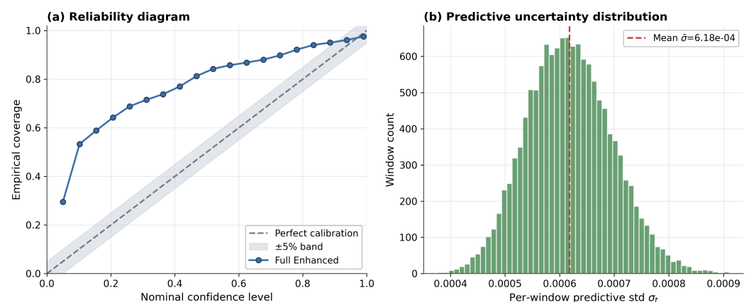
Figure 7. Uncertainty calibration on the held-out test split. (a) Reliability diagram (empirical coverage vs. nominal confidence; the diagonal is perfect calibration, below it is over-confidence). (b) Histogram of per-window predictive standard deviation \sigma_t ( M = 50 ), centred at \bar{\sigma} = 6.18 \times 10^{-4} .
