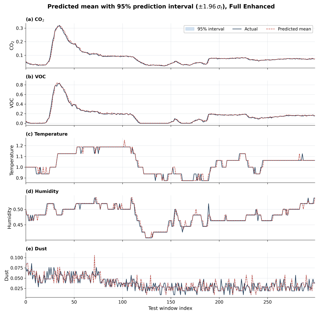
Figure 4. Predicted mean (solid) and 95% prediction interval (shaded band, \pm 1.96 \cdot \sigma_t ) from the Full Enhanced model on a representative test segment. The interval width adapts to per-window uncertainty: tighter during stable operation, wider during transient regimes.
