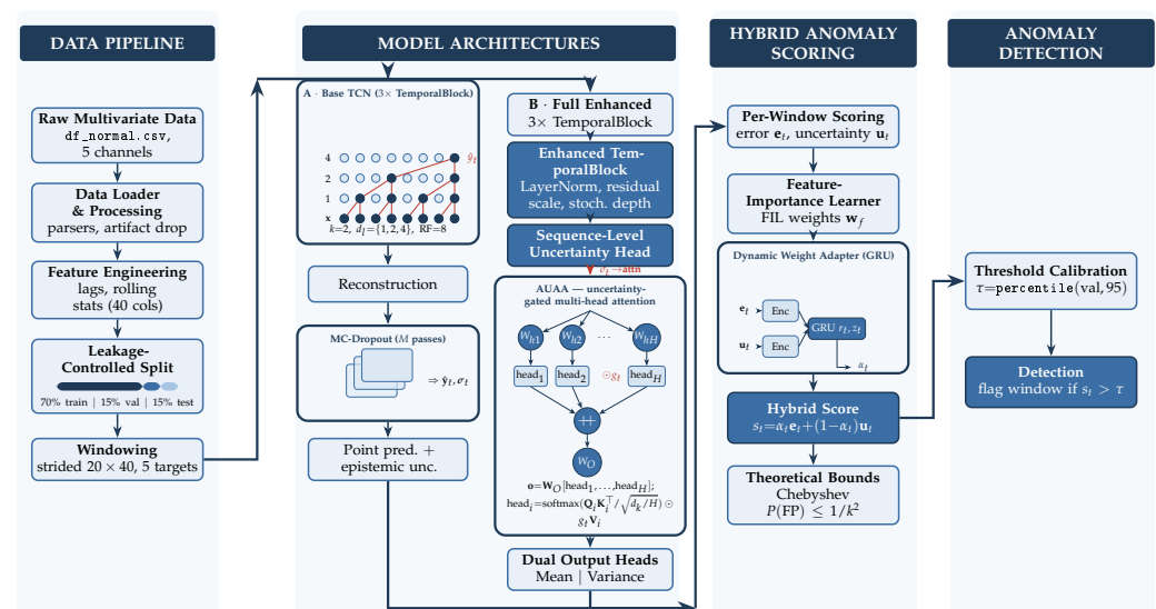
Figure 1. End-to-end architecture of the proposed uncertainty-aware TCN framework, organised as a four-stage pipeline: Data Pipeline (loading, leakage-controlled split, windowing) → Model Architectures (Base TCN and Full Enhanced) → Hybrid Anomaly Scoring → Anomaly Detection . The key backbone components are broken down inline: the Base TCN’s dilated causal convolution stack (kernel k=2 , dilations d_l=\{1, 2, 4\} , receptive field RF=8 ); the red path traces the dilated dependencies feeding the output \hat{y}_t , MC-dropout inference ( M stochastic passes \Rightarrow predictive mean \hat{y}_t and per-sensor epistemic \sigma_t ), the AUAA (4-head attention element-wise modulated by the uncertainty gate g_t=1/(1+\sigma_t) ), and the Dynamic Weight Adapter (GRU over e_t, u_t producing the learned weight \alpha_t ). Dark boxes mark the framework’s contributed components; the dashed red arrow marks the uncertainty-to-attention coupling that distinguishes this work from approaches that apply uncertainty only post hoc; detection via validation-calibrated thresholding terminates the pipeline.
