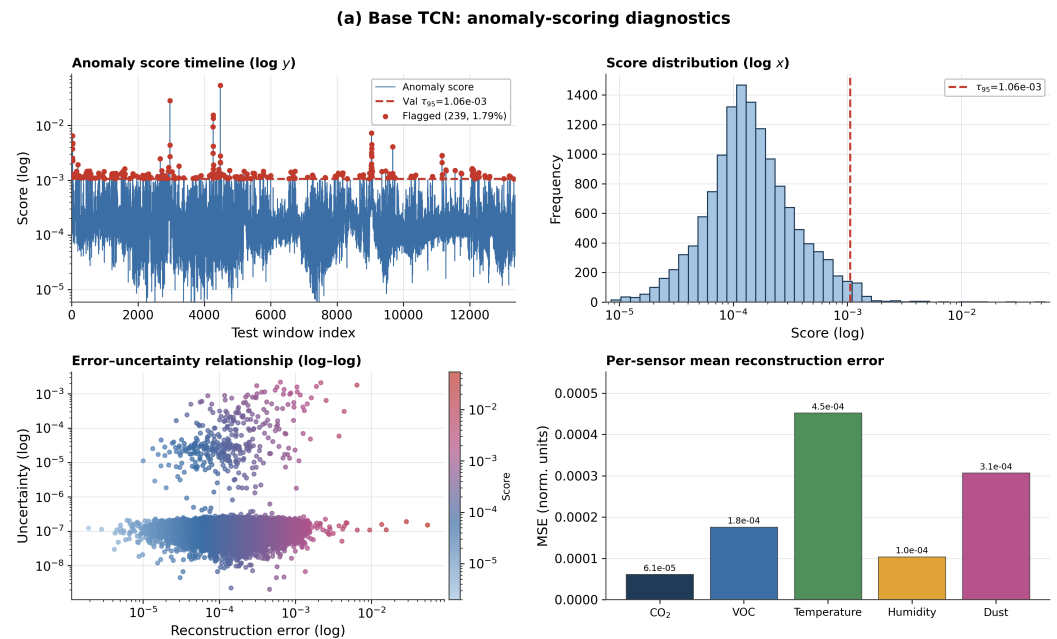
(a) Base TCN: \tau_{95} = 1.06 \times 10^{-3} , 239 flagged (1.79%).
