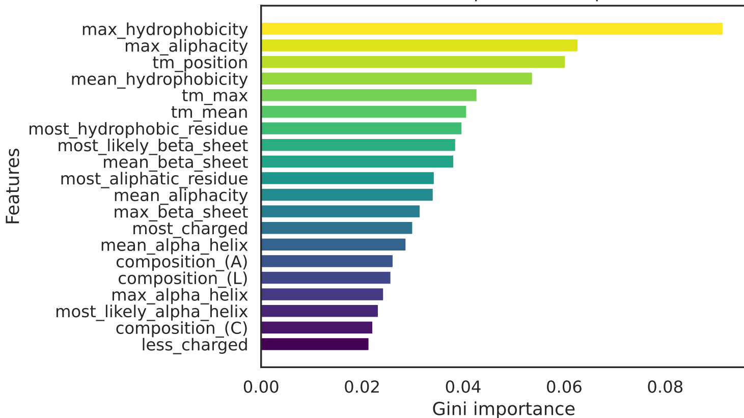
RandomForest Gini Importances (Top 20 - Round 4)
