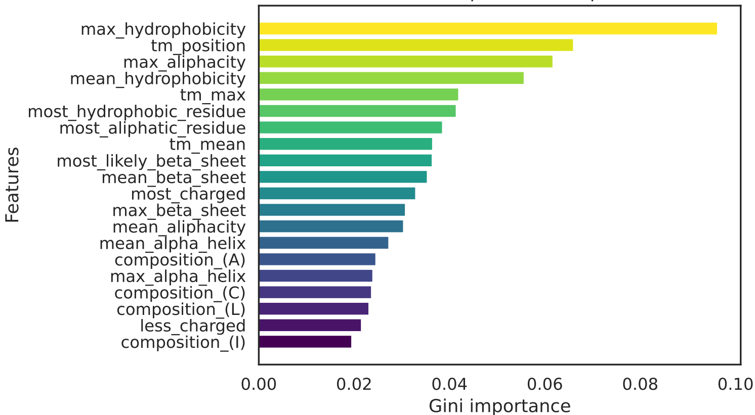
RandomForest Gini Importances (Top 20 - Round 5)
