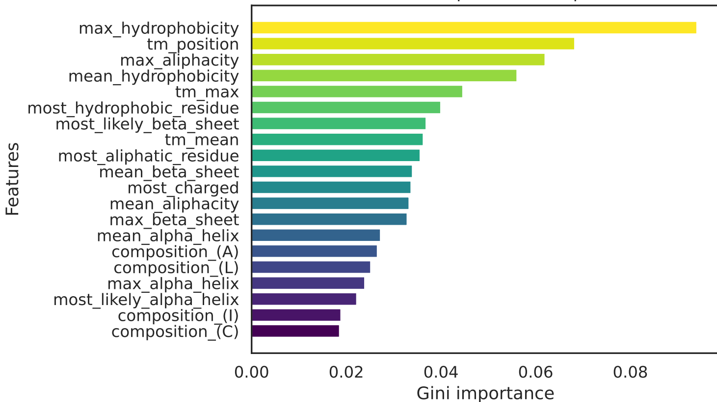
RandomForest Gini Importances (Top 20 - Round 1)
