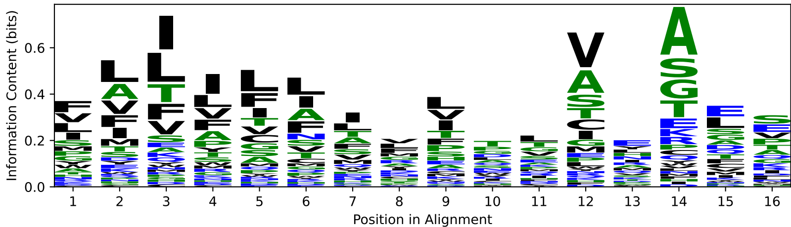
Sequence Logo
