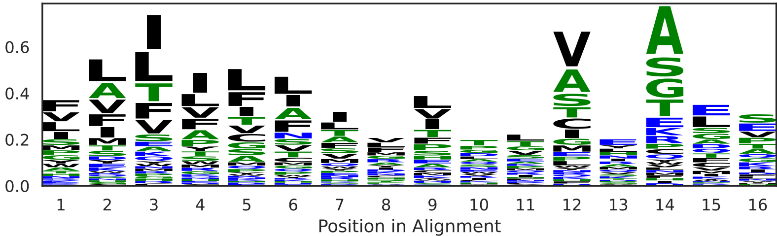
Sequence Logo
