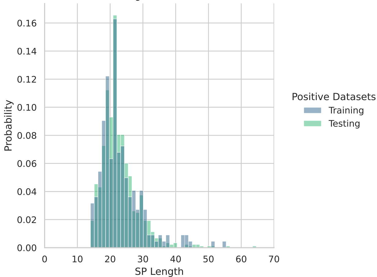
SP Length Distributions
