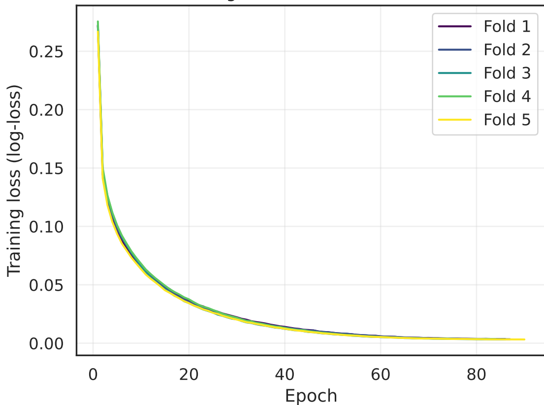
FFNN Training Curves (selected architecture)
