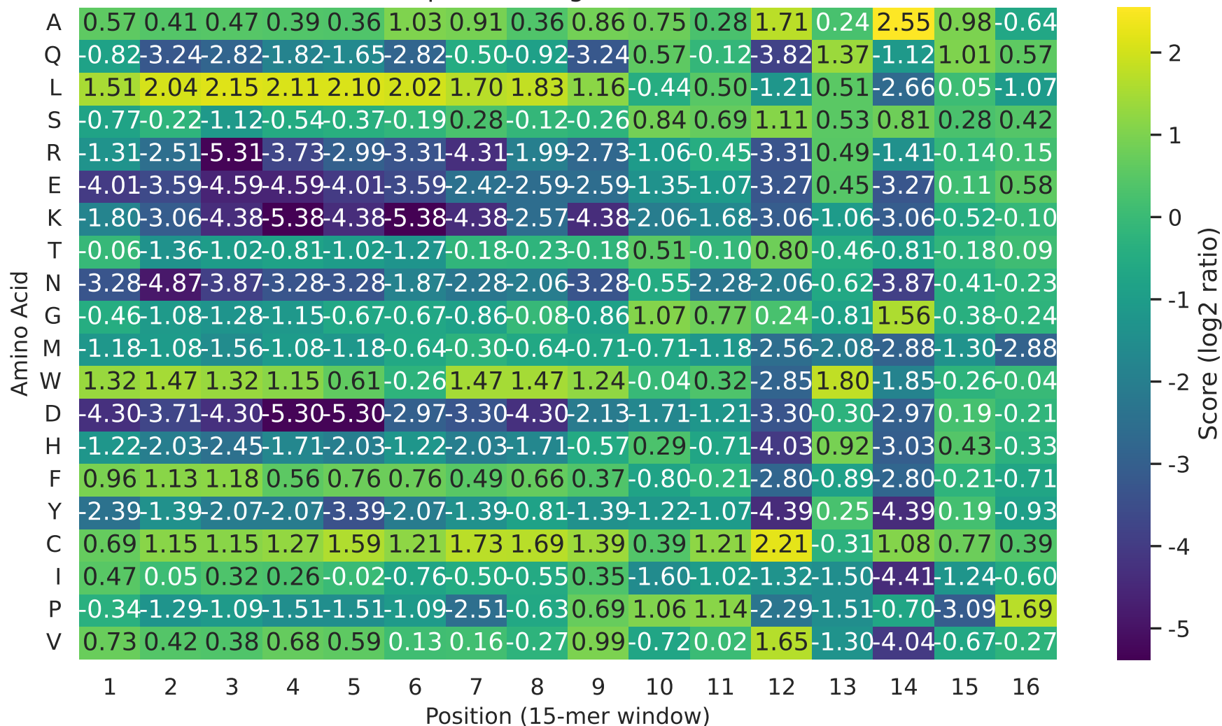
Position-Specific Weight Matrix (PSWM 3)
