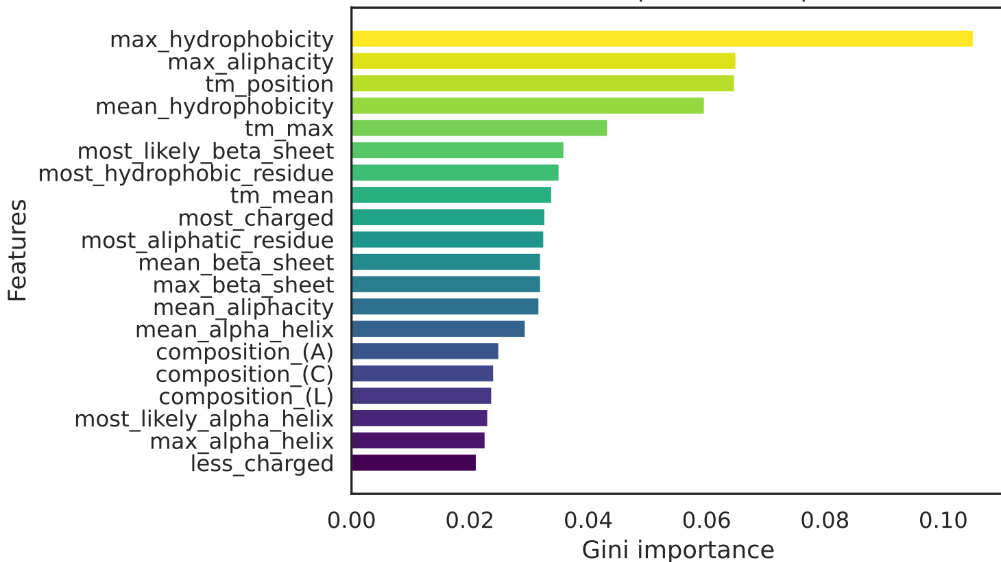
RandomForest Gini Importances (Top 20 - Round 2)
