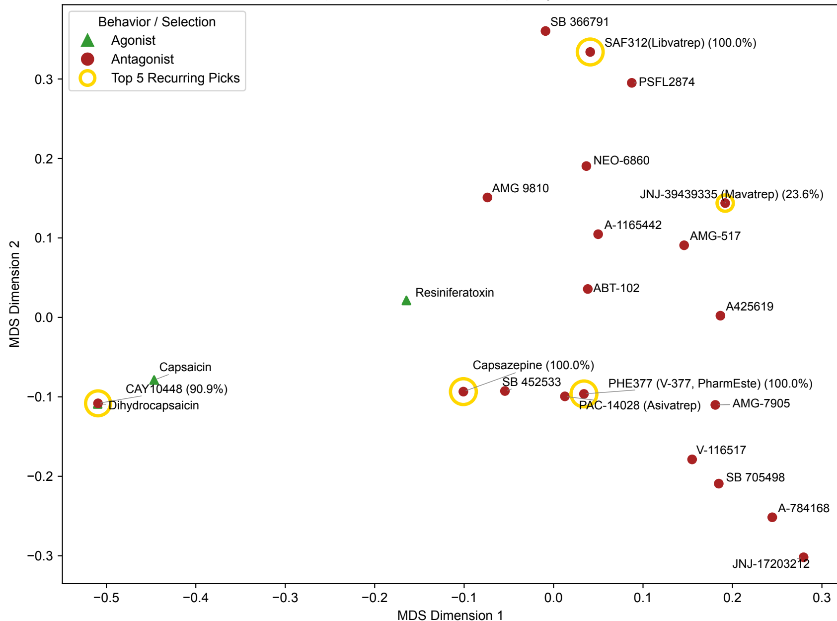
Classical MDS (MaxMax Selection Frequency over 1000 Seeds)
