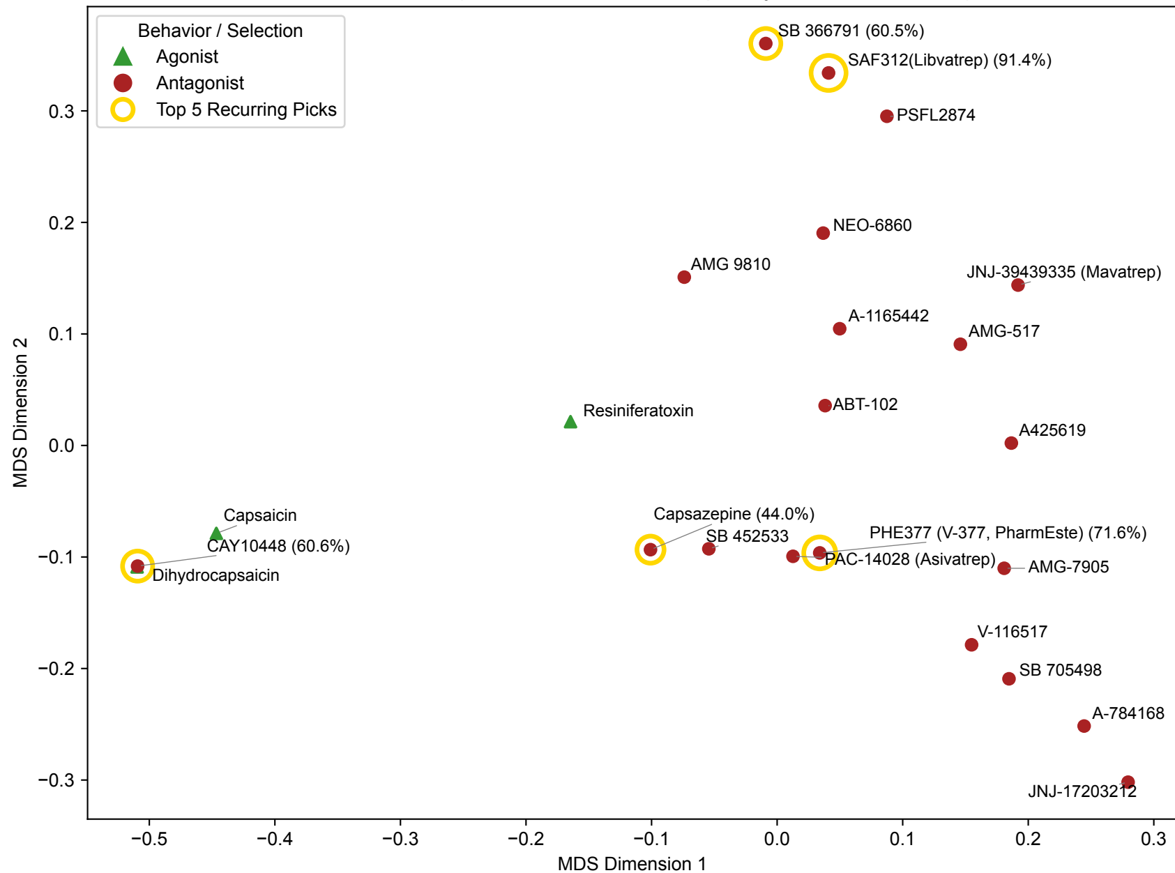
Classical MDS (MaxMin Selection Frequency over 1000 Seeds)
