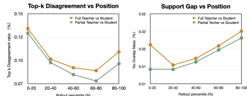
Figure A.2: Teacher-student support-gap diagnostics. Full-view targets show higher top- k disagreement and no-overlap mass than partial-view anchors across rollout positions.
