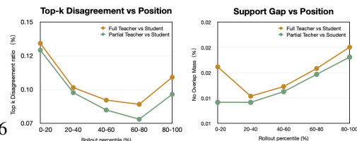
Figure A.2: Teacher-student support-gap diagnostics. Full-view targets show higher top- k disagreement and no-overlap mass than partial-view anchors across
