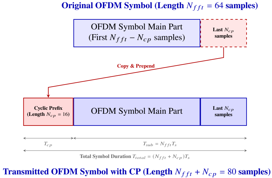
Figure 1: Cyclic Prefix (CP) Insertion Scheme in OFDM Symbol
