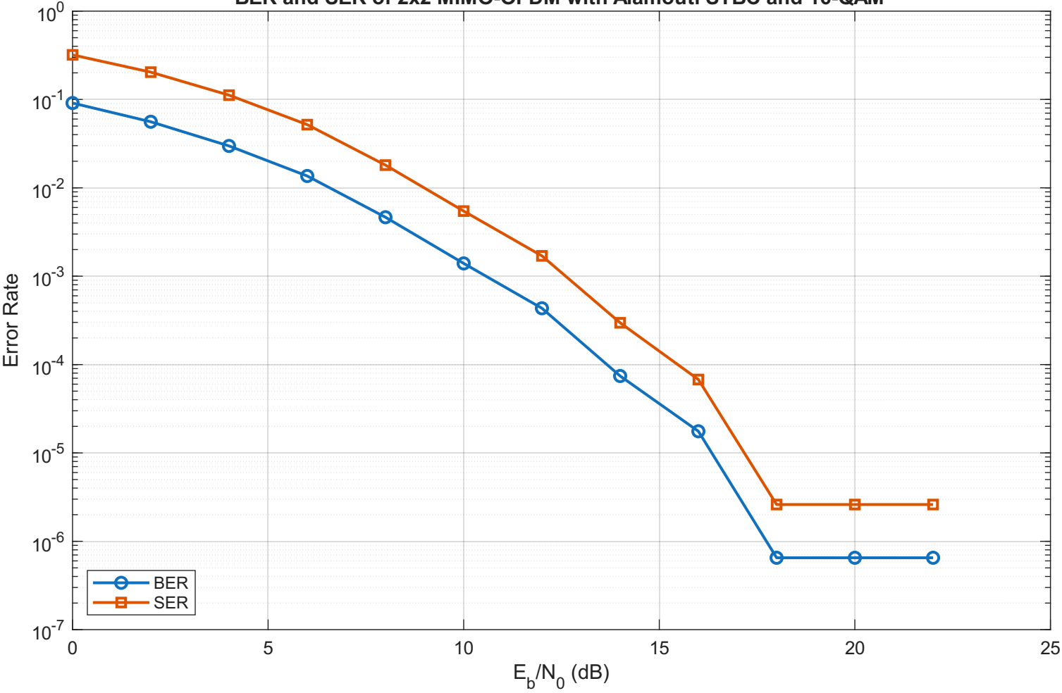
BER and SER of 2x2 MIMO-OFDM with Alamouti STBC and 16-QAM
