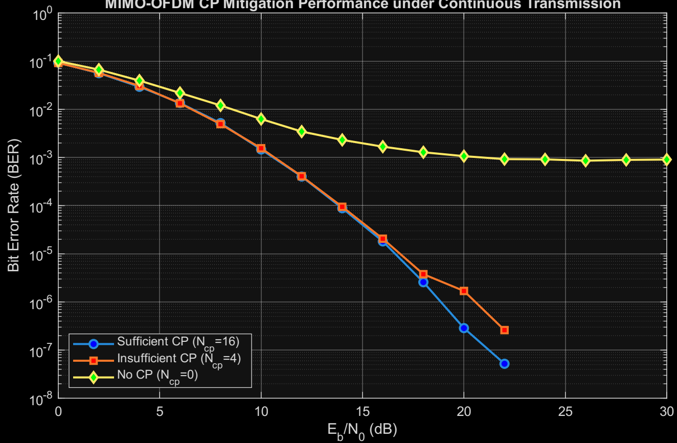
MIMO-OFDM CP Mitigation Performance under Continuous Transmission
