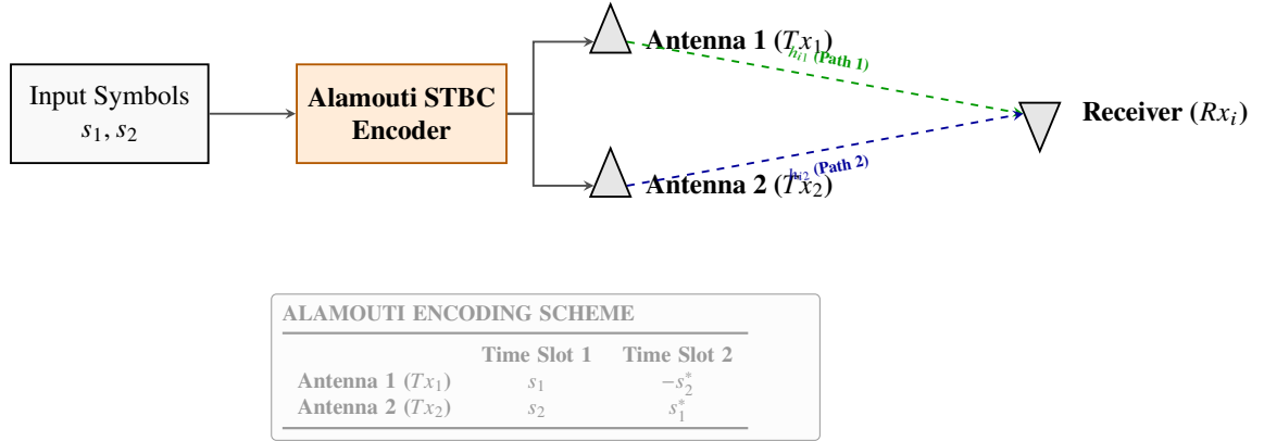
Figure 3: Alamouti Space-Time Block Coding Transmission Scheme
