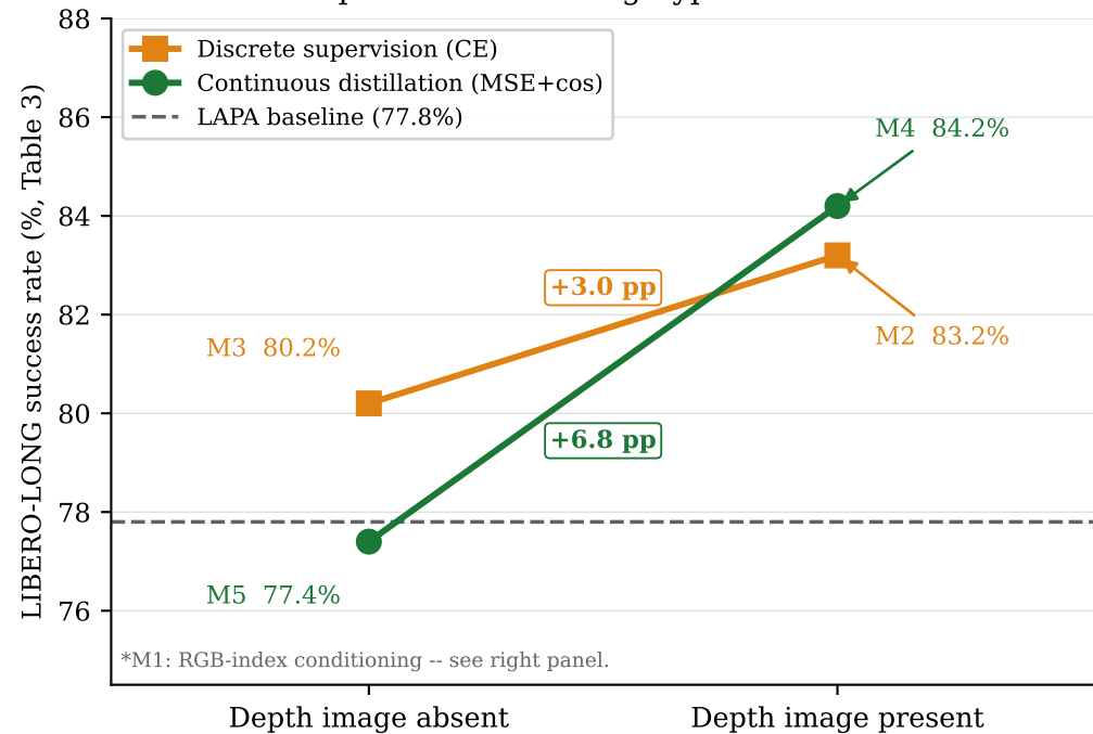
Depth × Conditioning Type Interaction
