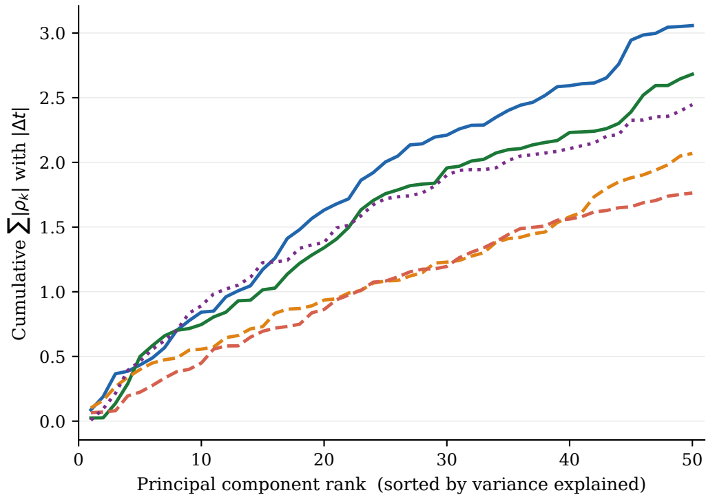
Geometric Signal Accumulation across PC Space (depth encoder output, 1024-d; top 50 PCs by variance)
