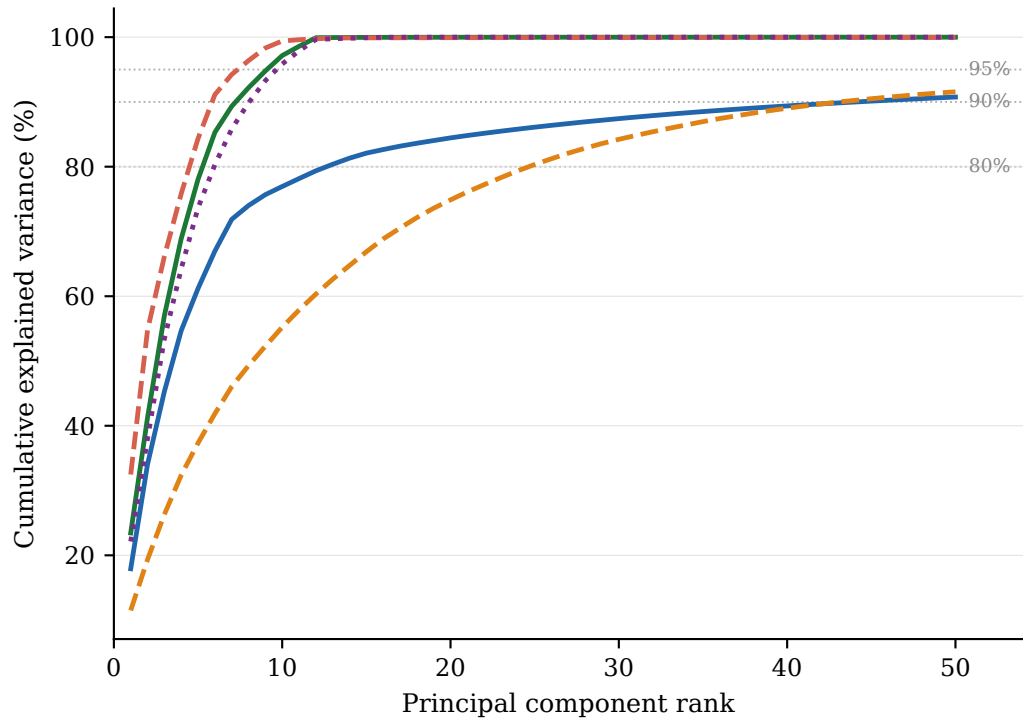
Variance Concentration (Scree) (how concentrated is the depth encoder's output variance?)
