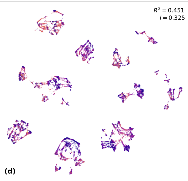
base LAPA ⊕ Model 3 (5120-d)
