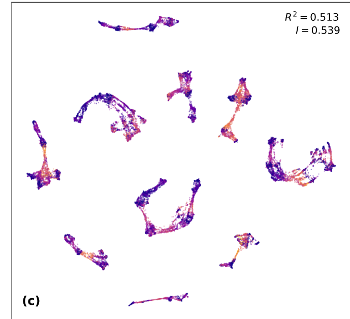
base LAPA ⊕ Model 2 (5120-d)
