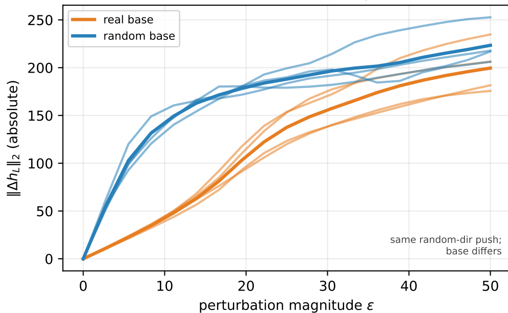
Tool-call windows: activation plateaus
