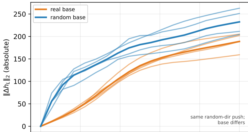
Prose windows: activation plateaus
