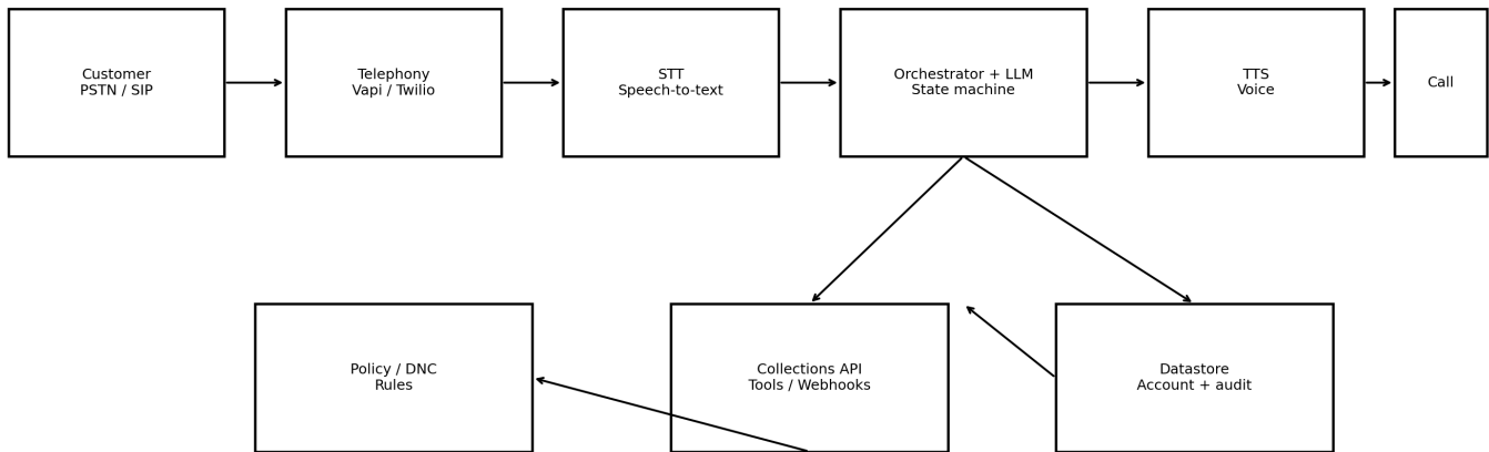
Kapture Finance Collections Voicebot — logical architecture
