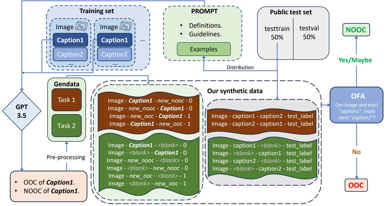
Figure 1: Pipeline of data processing and training the OFA model as our proposed End-to-end network.
