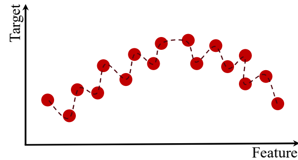
Overfitting
