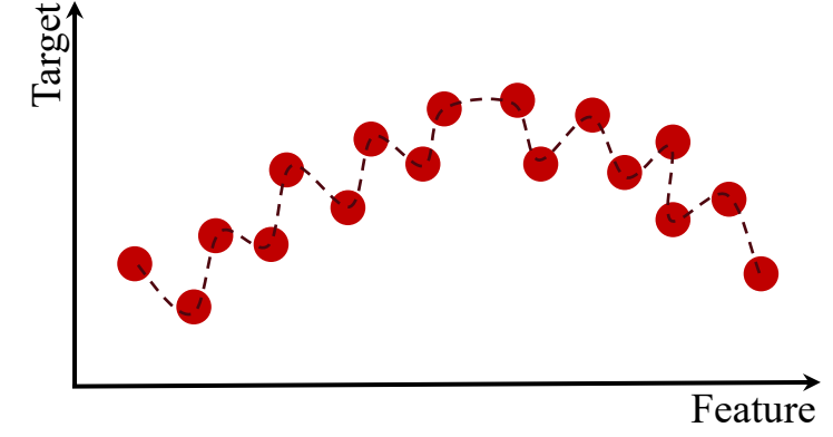
Overfitting
