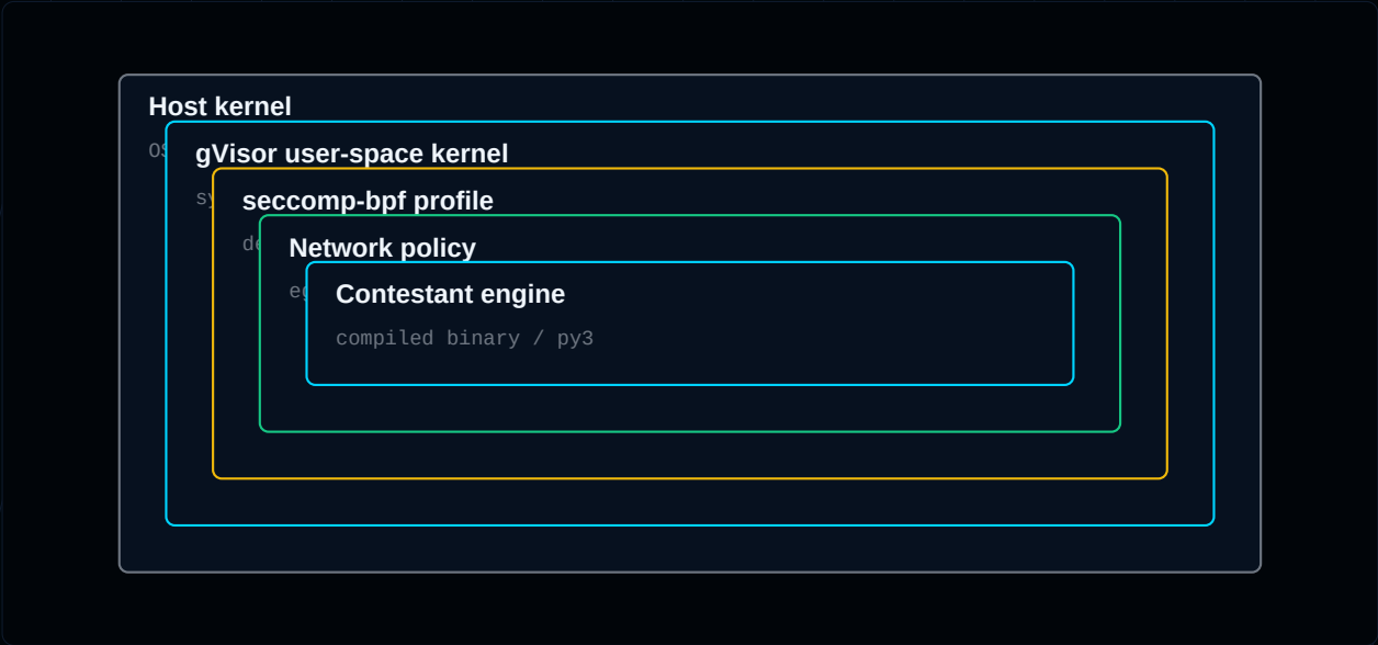
Figure 4 — Defense-in-depth around the contestant binary. The outermost rings are OS-level; the innermost is the code we don't trust.
