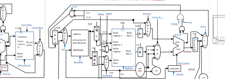
Multi-Cycle MIPS microprocessor's datapath
