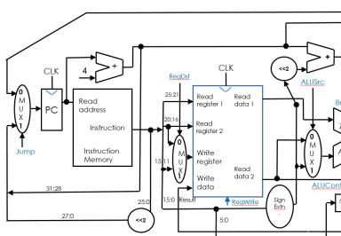
Single-Cycle MIPS microprocessor's datapath
