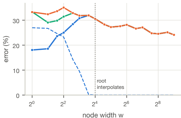
Cats vs Dogs, 20% label noise
