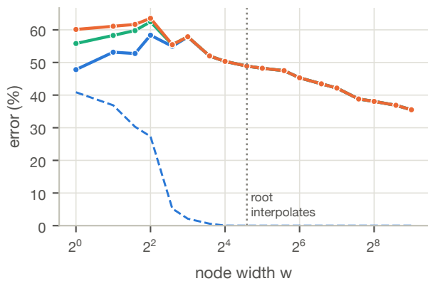
CIFAR-10, 20% label noise
