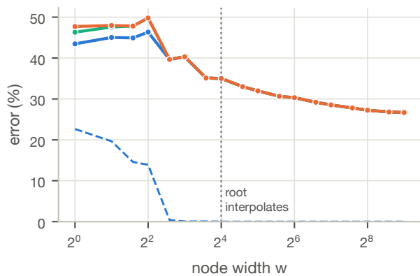
CIFAR-10, 0% label noise
